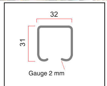
TRACK K-100 capacity 100 kg, standard length 6 m
