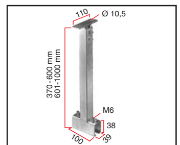
SOFFIT BRACKET KKS-100 370-600mm/601-1000 mm, adjustable
