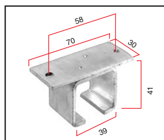
SOFFIT BRACKET KKK-100 Solid
