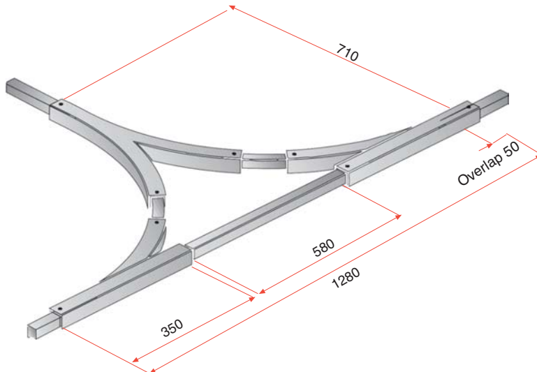
Three-way rail switch, complete ( 1x Y-rail switch, 1 x right rail switch, 1 x left rail switch + 2 x curve)
