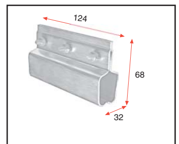
JOINT
