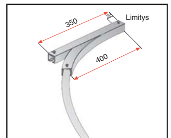
RAIL SWITCH
